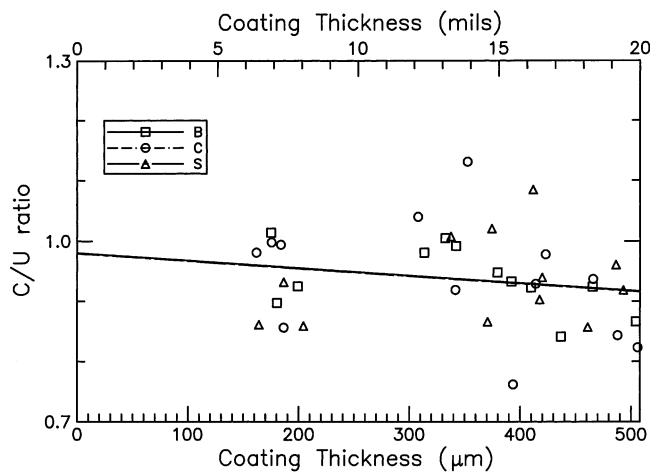
Fig. 5— C/U ratio versus coating thickness for coatings between 160 and 510 \mu\text{m} (6.4 to 19.9 mils).
