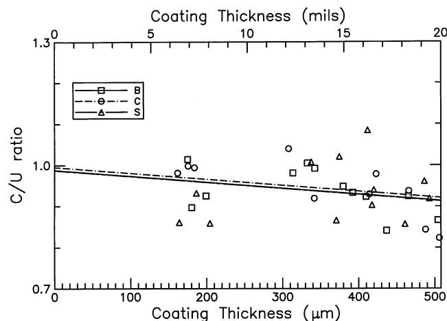
Fig. 6— C/U ratio versus coating thickness for coatings between 160 and 510 \mu\text{m} (6.4 to 19.9 mils), with unrepresentative test results removed.
