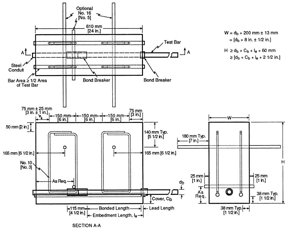
Fig. 1—Beam-end test specimen (ASTM A 944).
