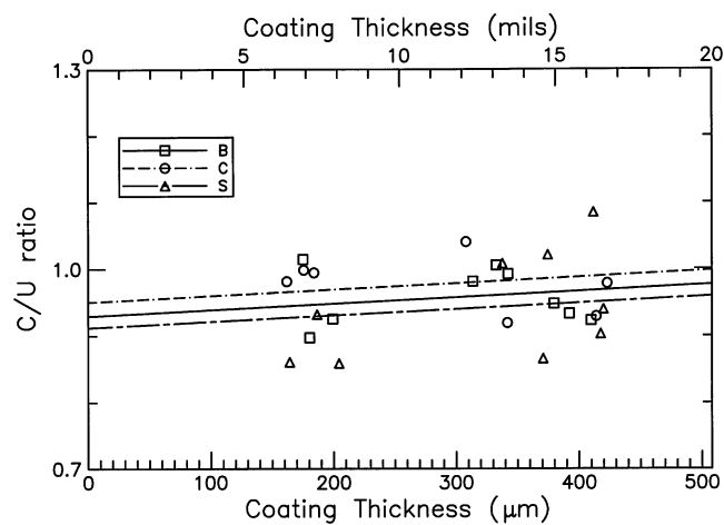
Fig. 7— C/U ratio versus coating thickness for coatings between 160 and 420 \mu\text{m} (6.4 to 16.5 mils).
