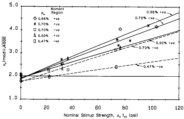
Fig. 11—Nominal shear stress normalized to concrete strength, v_n(\text{mod})/\sqrt{4000} , versus \rho_v f_{vy} ( 1000 \text{ psi} = 6.895 \text{ MPa} )
