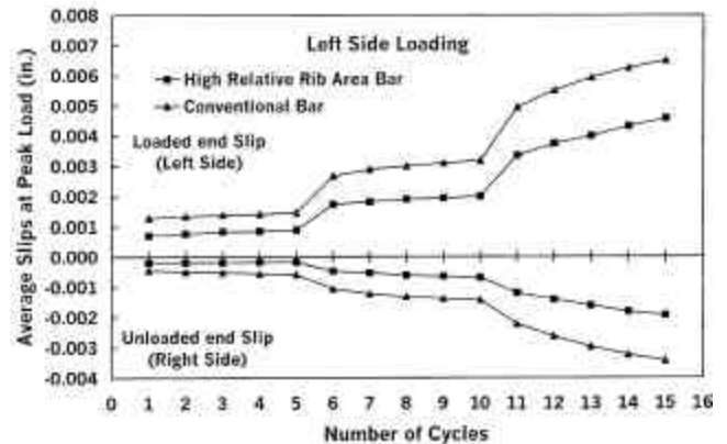
Fig. 4—Average slips of conventional bars 3, 5, 7, 9, and 11 and high relative rib area bars 4, 6, 8, and 10 at peak loads versus number of loading cycles for left side loading (1 in. =
