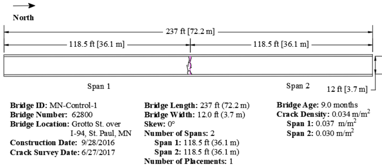
Figure G.4: Crack Map for MN-Control-1 (Survey 1)
