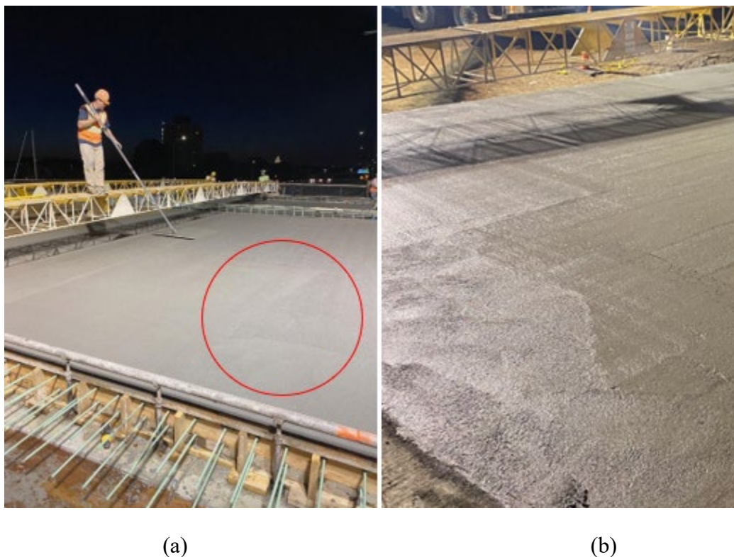
Figure 4.23: Bullfloating the deck in the presence of bleed water (a) an overview; (b) a close-up view
