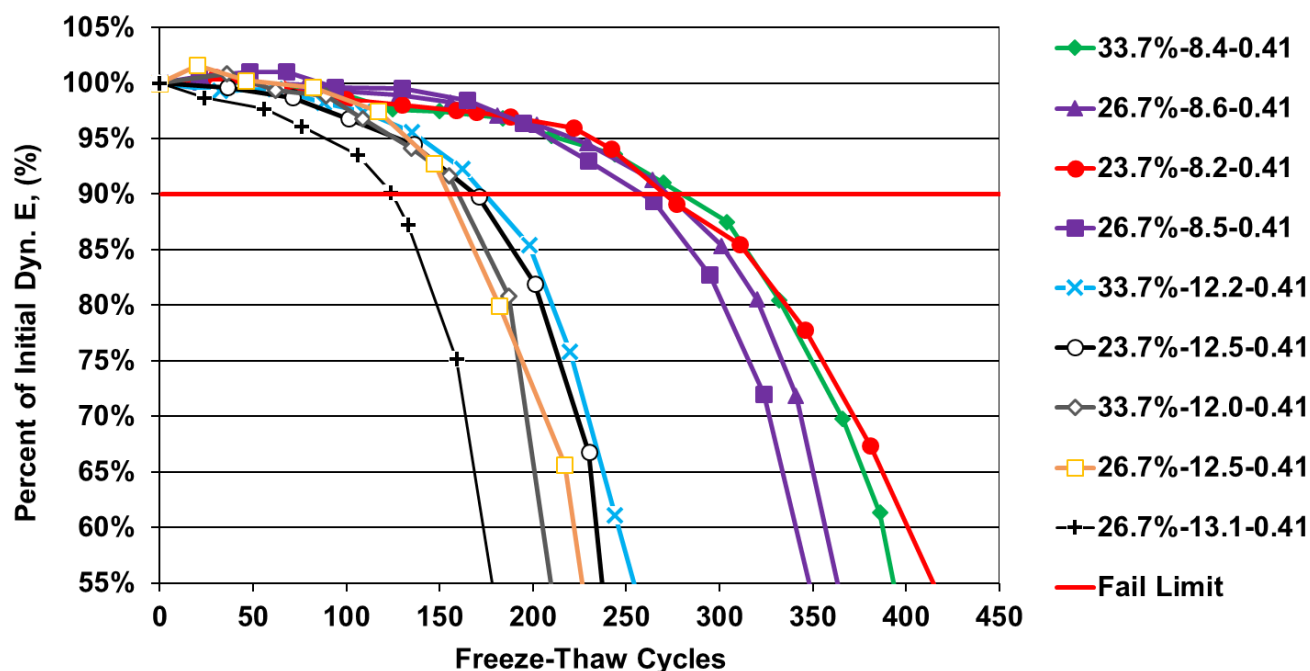
Figure 3.2: Average percent of initial dynamic modulus of elasticity vs. freeze-thaw cycles for mixtures with a w/c ratio of 0.41 tested in accordance with ASTM C666-Procedure A
