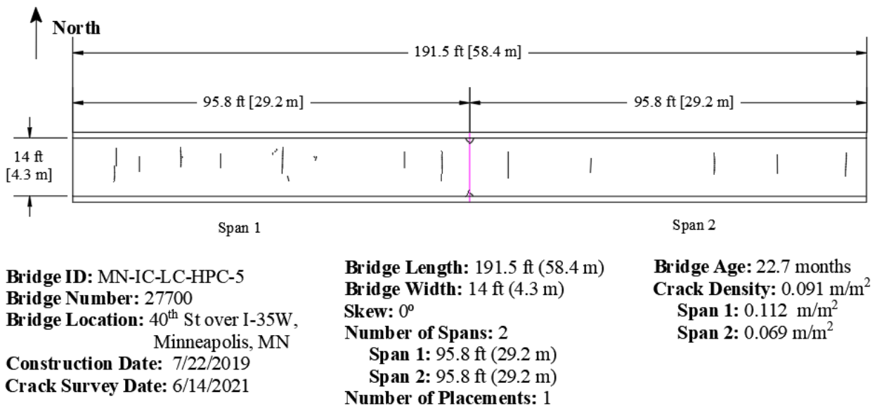
Figure 5.14: Crack map for MN-IC-LC-HPC-5 (Survey 2)
