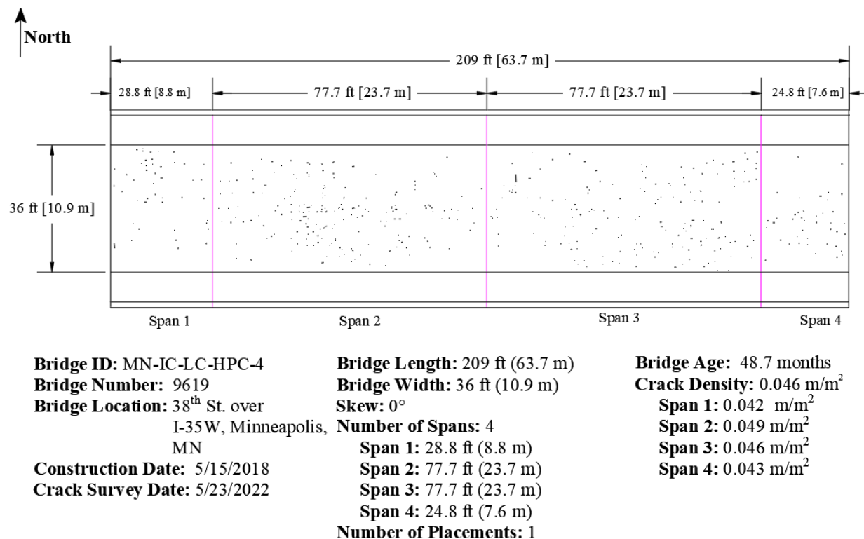
Figure 5.12: Crack map for MN-IC-LC-HPC-4 (Survey 3)
