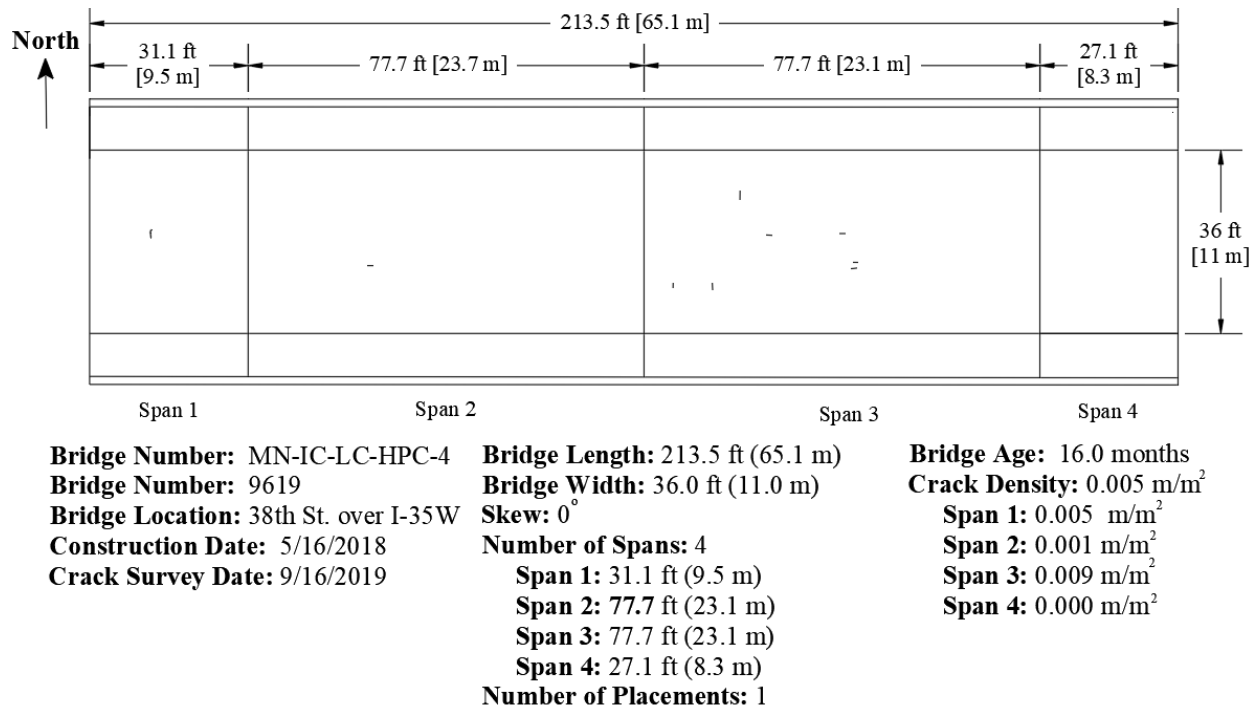
Figure G.13: Crack Map for MN-IC-LC-HPC-4 (Survey 1)
