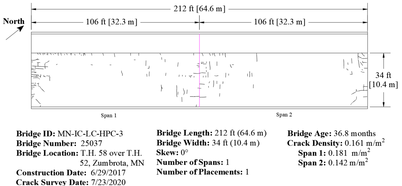
Figure 5.10: Crack map for MN-IC-LC-HPC-3 (Survey 3)
