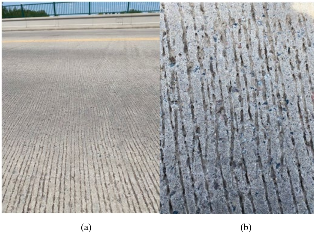
Figure 5.20: Poorly tining of MN-IC-LC-HPC-6 (a) an overview; (b) a close-up view
