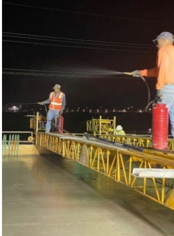
Figure 4.66: Applying finishing aid to the concrete surface
