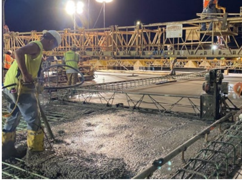
Figure 4.21: Placement equipment
