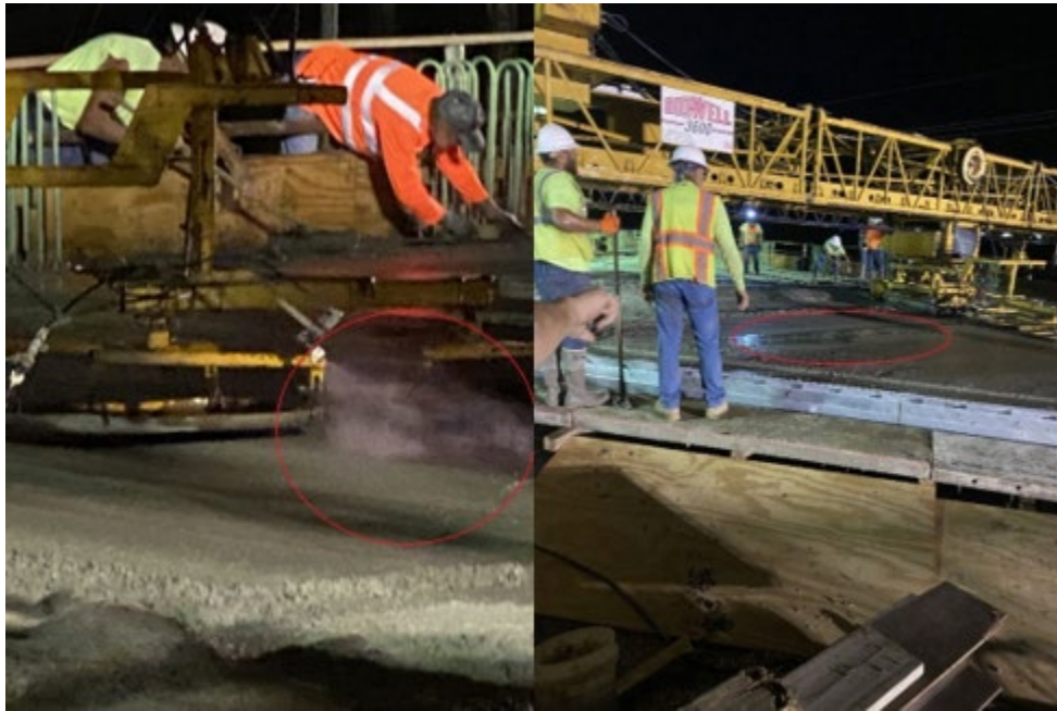
(a) (b) Figure 4.64: Excessive water on the deck (a) not adjusted nozzles; (b) ponded water on the surface
