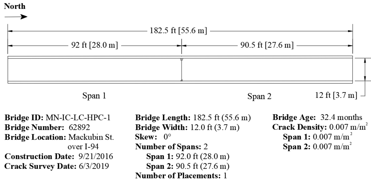
Figure G.3: Crack Map for MN-IC-LC-HPC-1 (Survey 3)
