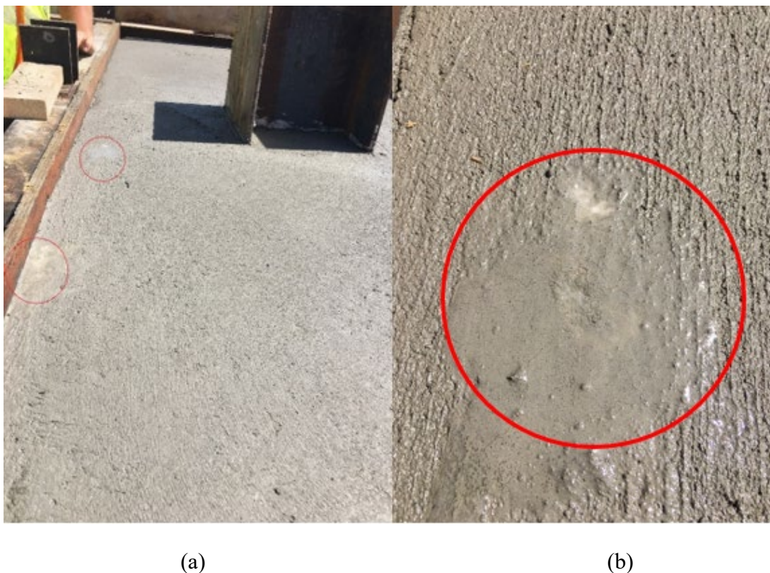
Figure 4.27: Small trapped air pockets at edges of third trial placement (a) overview; (b) close-up (image provided by MnDOT)
