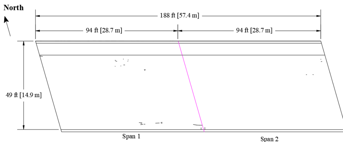
Figure 5.18: Crack map for MN-IC-LC-HPC-6 (Survey 2)
