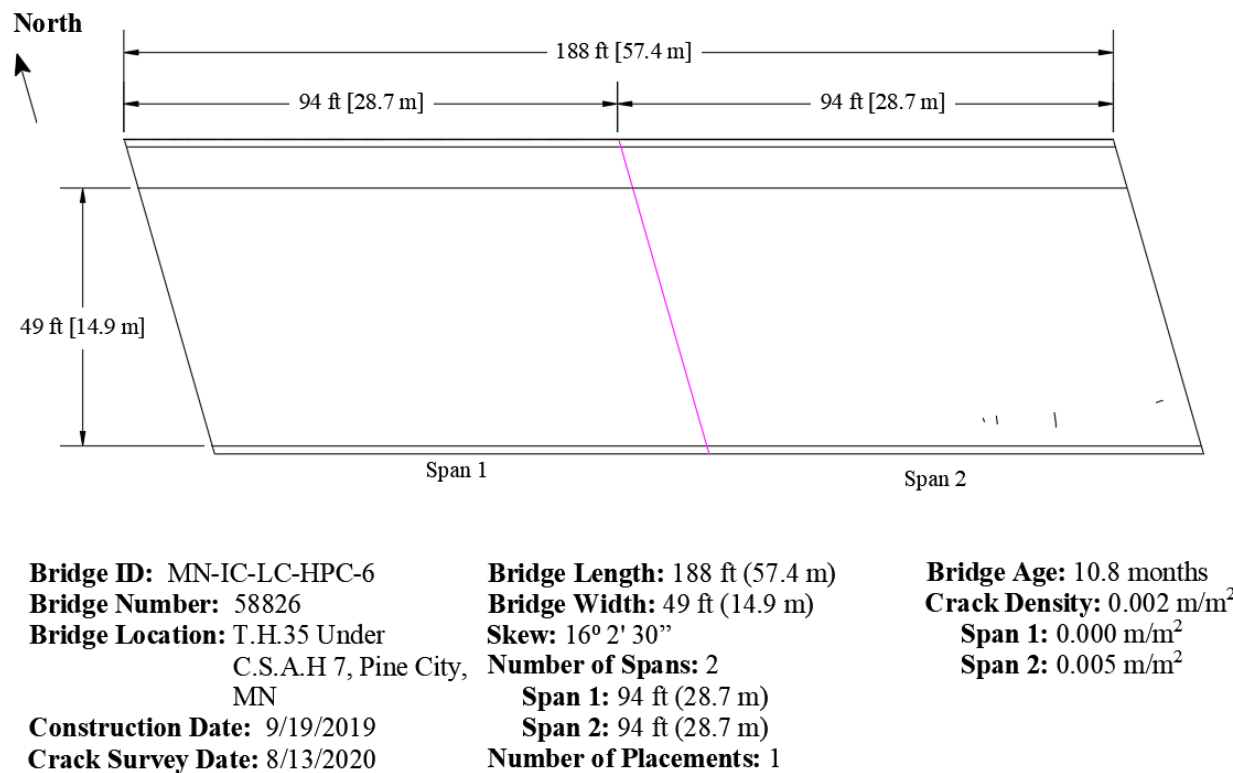
Figure 5.17: Crack map for MN-IC-LC-HPC-6 (Survey 1)
