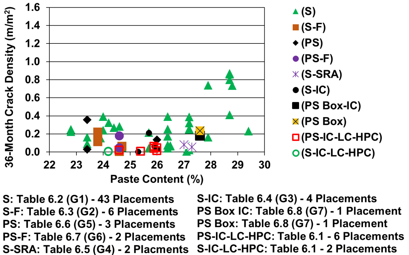
Figure 6.1: Paste content versus 36-month crack density for decks with good construction practices-Decks described in Tables 6.1 to 6.8
