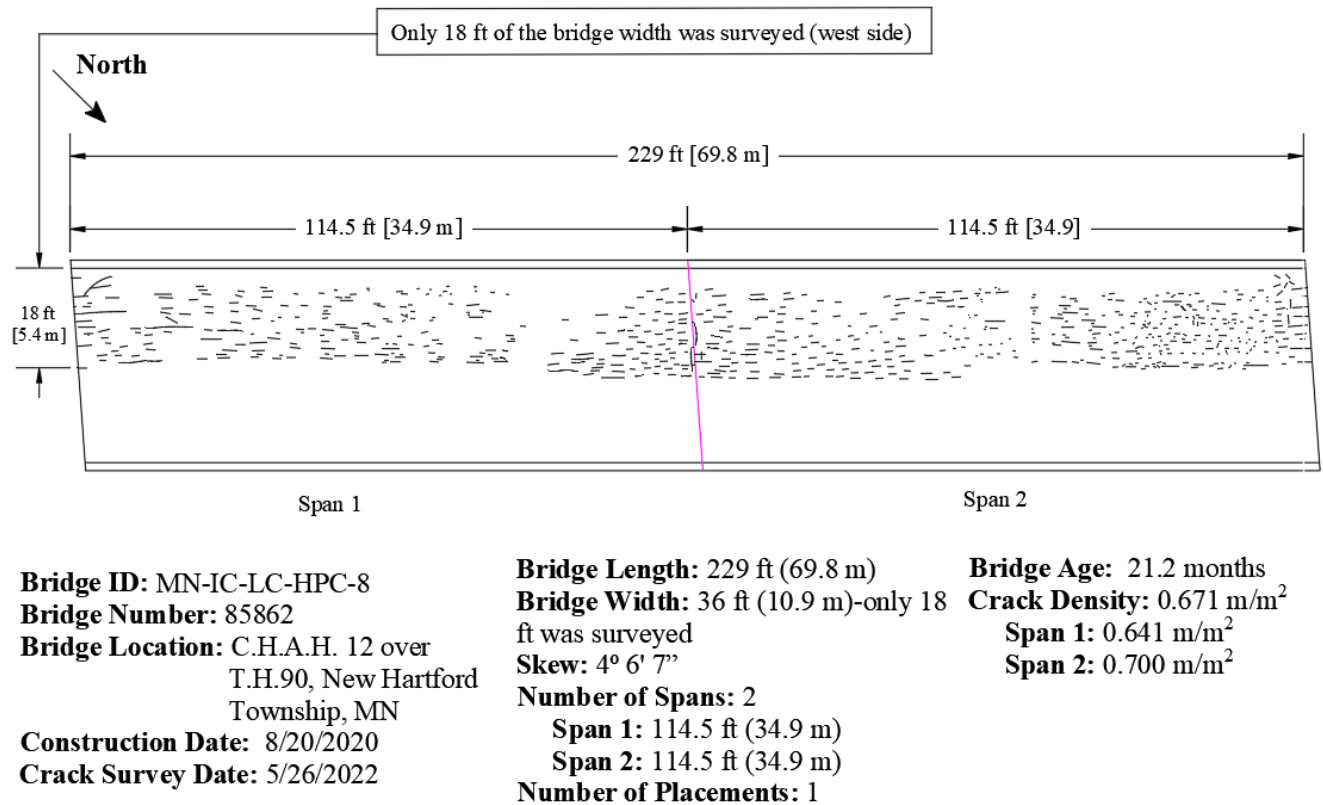
Figure 5.25: Crack map for MN-IC-LC-HPC-8 (Survey 2)
