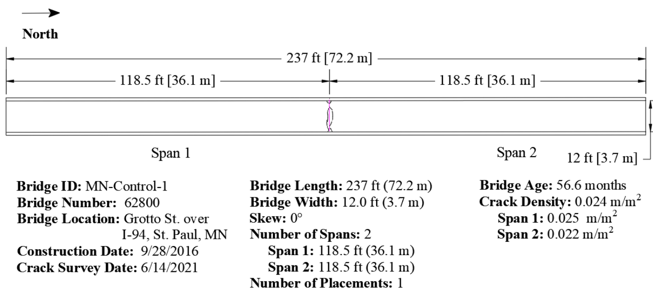
Figure 5.6: Crack map for MN-Control-1 (Survey 5)
