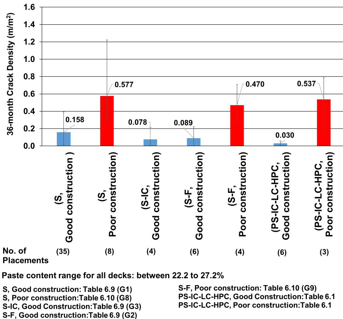
Figure 6.6: Comparing the 36-month crack densities of decks with good vs. poor construction practices
