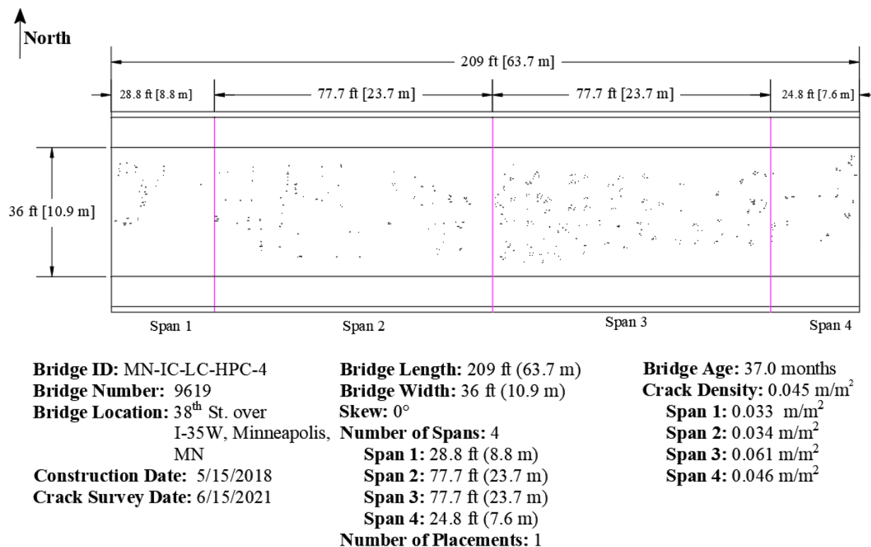
Figure 5.11: Crack map for MN-IC-LC-HPC-4 (Survey 2)
