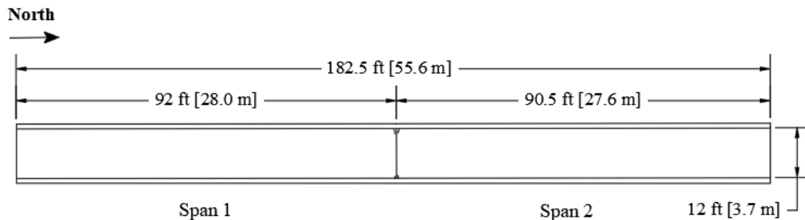
Figure G.1: Crack Map for MN-IC-LC-HPC-1 (Survey 1)
