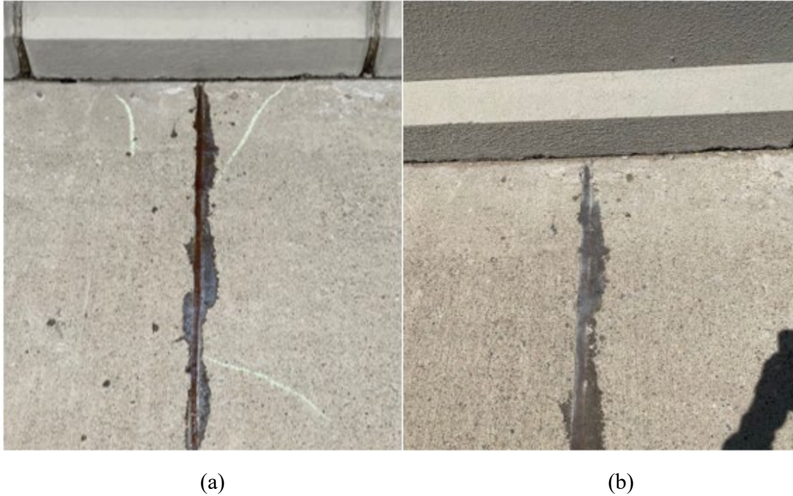
Figure 5.1: Comparison of the center pier of MN-IC-LC-HPC-1 (a) from Survey 5; (b) from Survey 6
